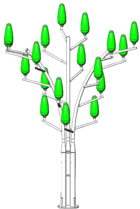
MODULAR TREE , regular or hybrid 18, 24 or 30 Aeroleaf / 12, 16, 20 solar petals
